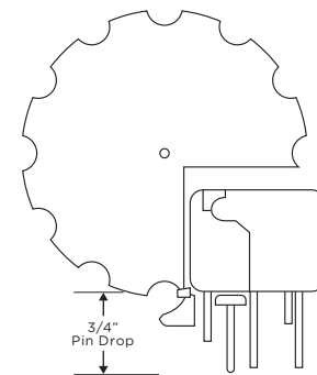
3 Inch Wood Traverse or Ripplefold Rod
