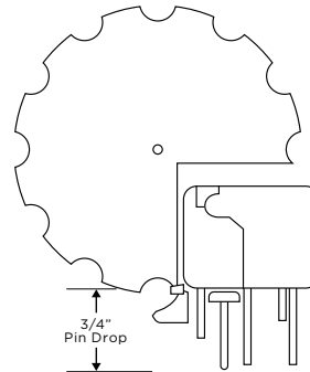
3 Inch Wood Traverse or Ripplefold Rod
