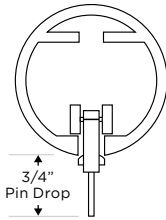
1-3/4 Inch Metal Zip Rod with Zip Eyelets
