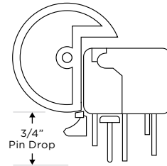
1-3/4 Inch Metal Traverse or Ripplefold Rod
