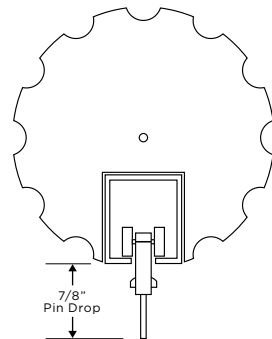
3 Inch Wood Zip Rod with Zip Eyelets
